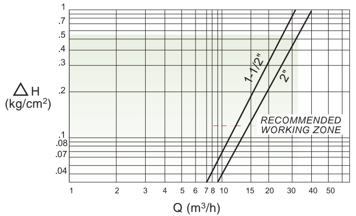
Head loss for fully open valve
